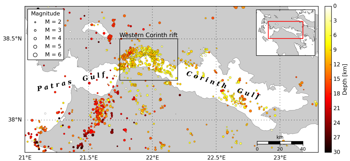
Figure 4.24 – Microseismicity map recorded by the NOA network in the Patras Gulf and the Corinth Gulf. The magnitude M > 2 earthquakes from 2006 to 2015 are shown. The colors represent the event depth.
