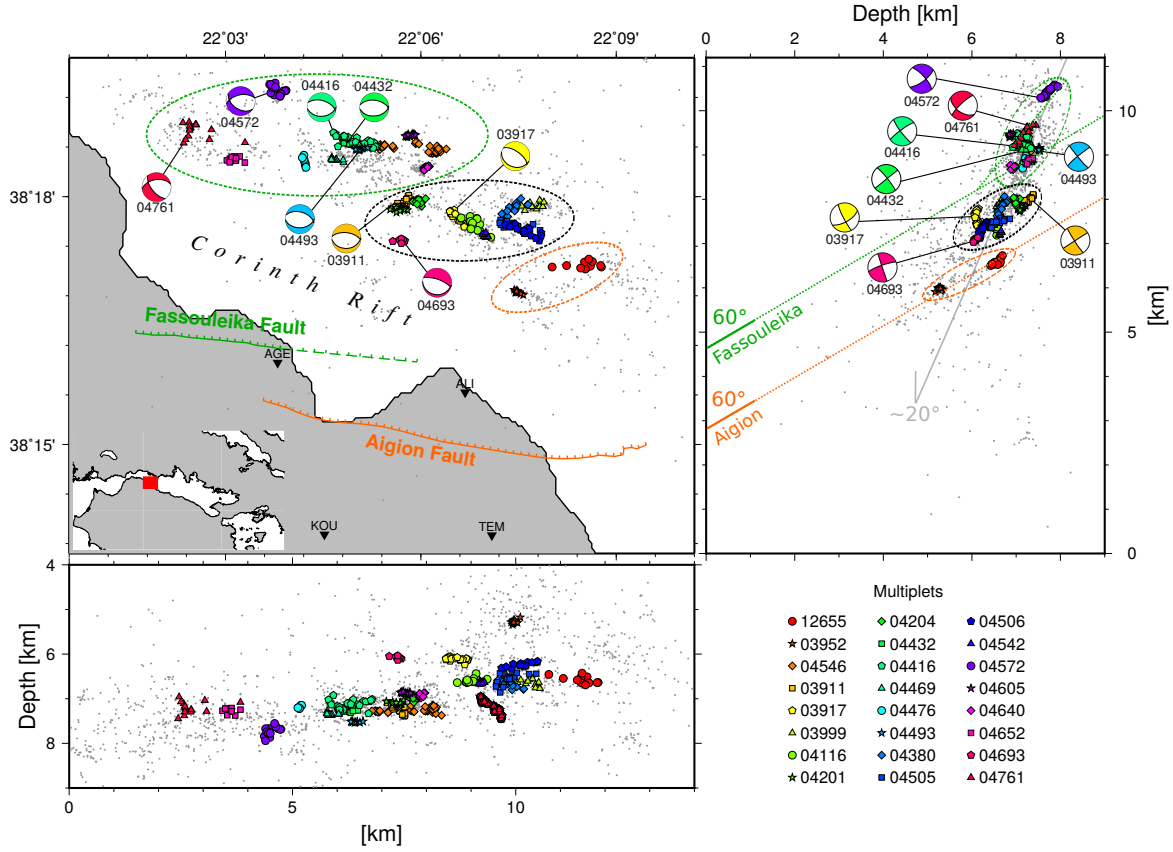
Figure 3.2 – Map, EW and NS vertical sections of the 2003–2004 swarm. The 24 main multiplets have specific colored symbols. The background microseismicity is represented as gray dots. The Aigion and Fassoileika faults dipping about 60° at surface are the two main structures illuminated at depth by respectively 2 (dashed orange ellipses) and 11 (dashed green ellipses) multiplets. A third structure (dashed black ellipses) between these faults is highlighted by the remaining multiplets and assimilated to a relay zone. Focal mechanisms are from Godano et al. [2014] .
