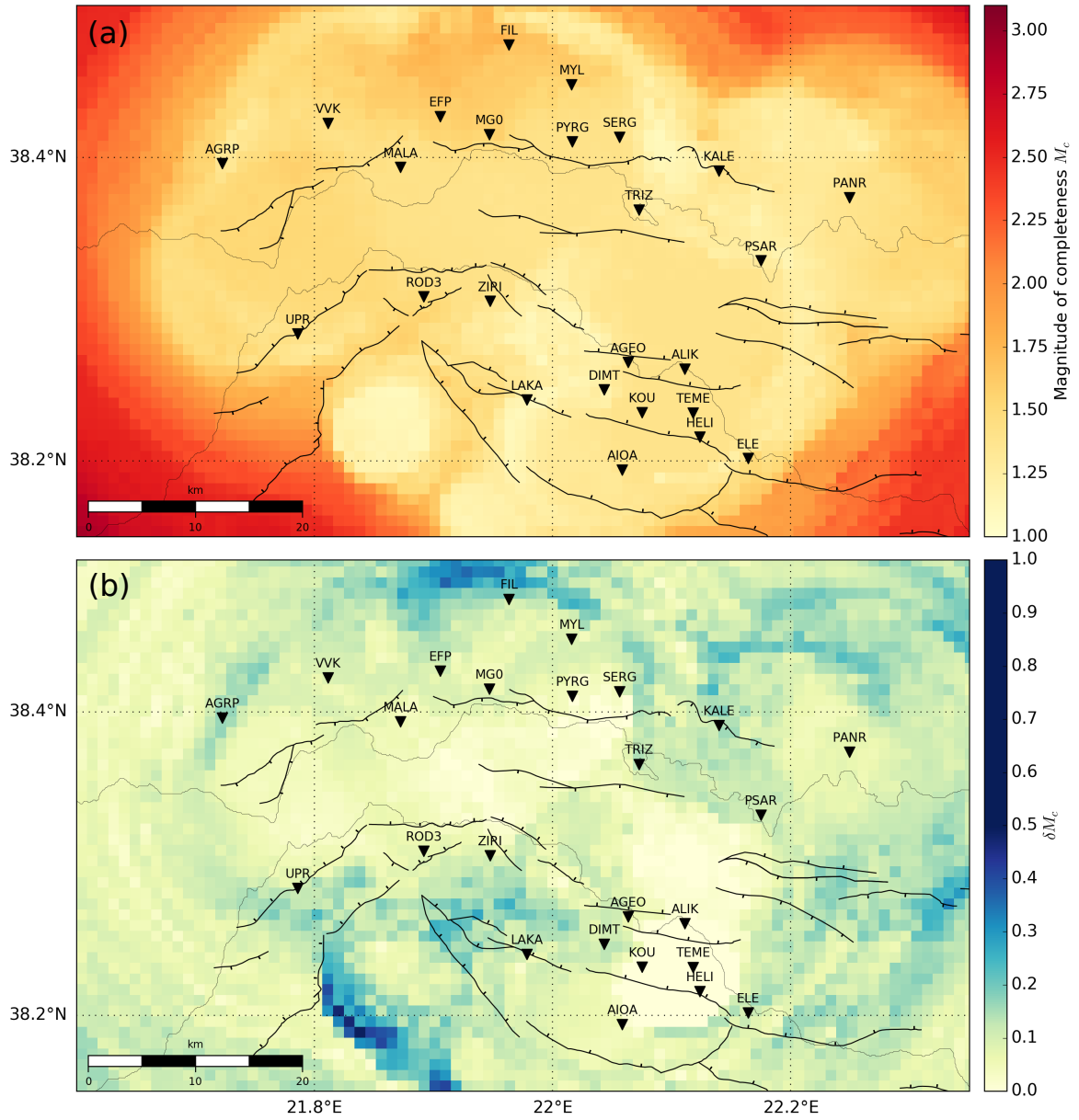
FIGURE C.2 – Spatiiale variation of the completeness magnitude over the Corinth rift. (a) Map of completeness magnitude M_c . (b) Map of the uncertainty \delta M_c . The main normal faults are represented by black lines. Some stations are shown as visual marks with upside down black triangles.
