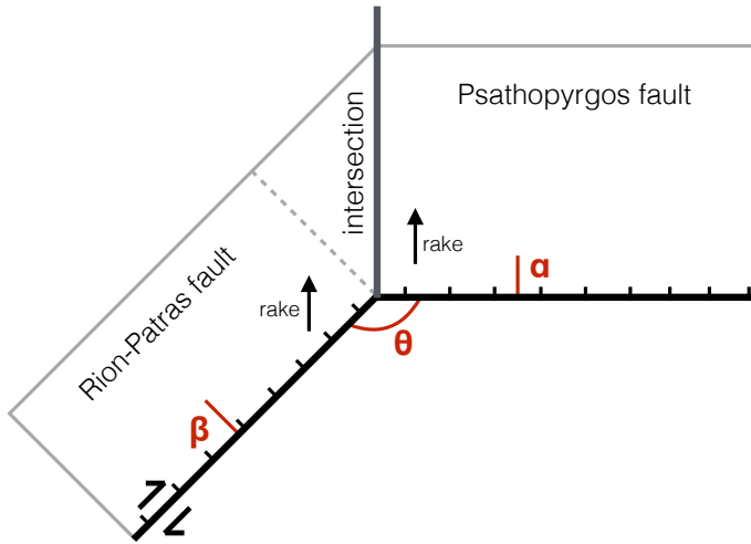
Figure 4.23 – Geometry of the depth contact between the Psathopyrgos and the Rion-Patras faults. \alpha is the dip angle of the Psathopyrgos fault. \beta is the dip angle of the Rion-Patras fault. \theta is the angle at the surface between the two fault extension ( \theta = 135^\circ ).
