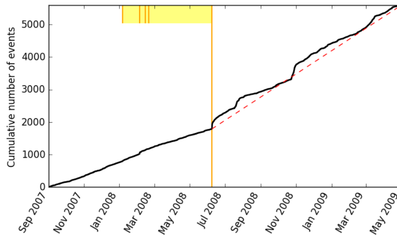
Figure 5.11 – Cumulative number of M_W \geq 1.2 events recorded by the CRL network between 2007 and 2009. As in Durand et al. [2014], we observed the change in the seismicity rate at large temporal scale after the sequence of M > 6 earthquakes in Greece. The yellow colored slot indicates the duration of this sequence and the orange vertical lines their occurrence time.
