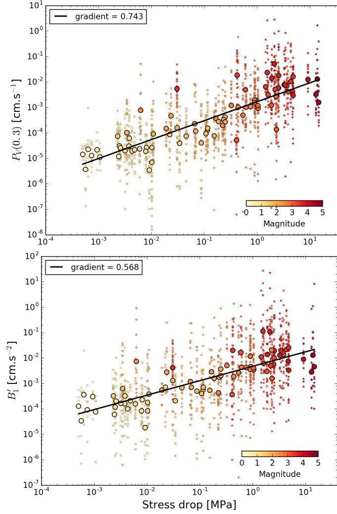
Figure 6.10 – Peak velocity measurements as a function of the stress drop. (a) The circles are the average peak velocity by event at 0.3 s after the P-arrival time P_V(0.3) ( \text{cm.s}^{-1} ) as a function of \sigma (MPa). (b) The circles are the slope B'_1 ( \text{cm.s}^{-2} ) as a function of \sigma (MPa). The stars are the data for each event at each station. The black lines are the best fit over the average data points. The gradient of these lines are estimated to \sim 0.7 for (a) and \sim 0.6 for (b).
