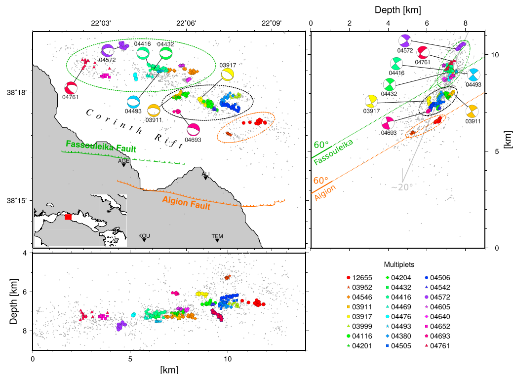
Figure 2. Map, EW, and NS vertical sections of the 2003–2004 swarm. The 24 main multiplets have specific colored symbols. The background microseismicity is represented as gray dots. The Aigion and Fassoouleika faults dipping about 60° at surface are the two main structures illuminated at depth by, respectively, 2 (dashed orange ellipses) and 11 (dashed green ellipses) multiplets. A third structure (dashed black ellipses) between these faults is highlighted by the remaining multiplets and assimilated to a relay zone. Focal mechanisms are from Godano et al. [2014].
