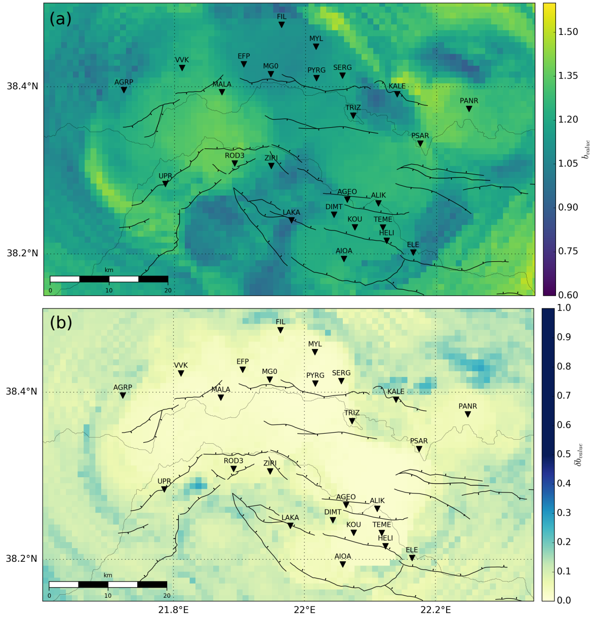
FIGURE C.3 – Spatiale variation of the b -value over the Corinth rift. (a) Map of the b -value. (b) Map of the uncertainty \delta b -value. Markers are the same as in the Figure C.2.
