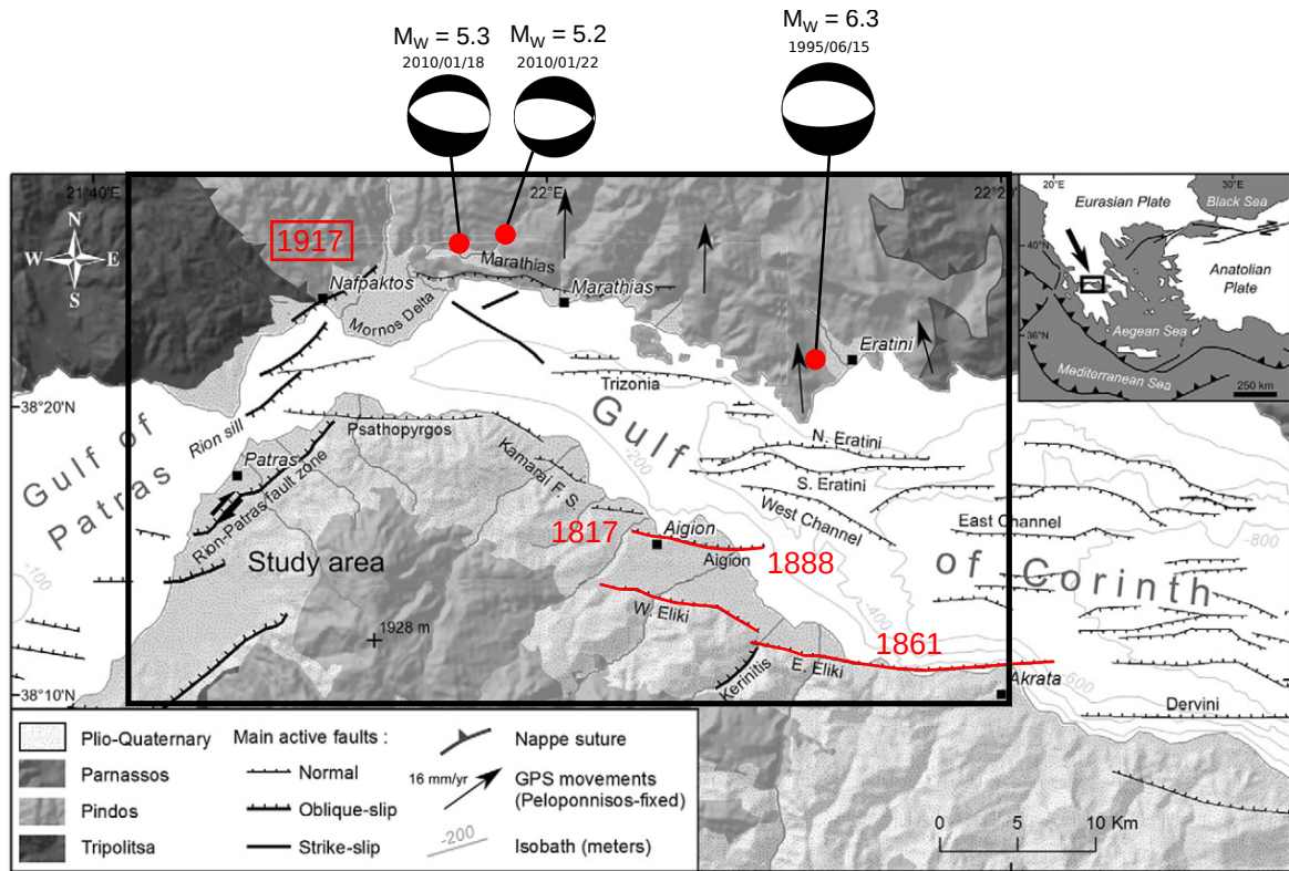
Figure 4.1 – Tectonic map of the central and western part of the Corinth rift. Onshore active faults are from Ford et al. [2013, 2009] ; Palyvos et al. [2008, 2005] , main offshore faults are from Beckers et al. [2015] ; Bell et al. [2009] ; Flotté et al. [2005] ; Taylor et al. [2011] . Isobaths are from Bell et al. [2008] and GPS measurements are from Avallone et al. [2004] . Epicenters and focal mechanisms of magnitude M > 5 earthquakes are from Bernard et al. [1997] ; Sokos et al. [2012] . Historical earthquakes of magnitude M \geq 6 affecting faults in the study area (black frame) are mentioned in red by dates [ Albini et al., 2017 ]. The distribution of the onshore Hellenide nappes and the Plio-Pleistocene sediments are drawn and described in the legend. The insert shows the Hellenic subduction in the south and the dextral detachment of the North Anatolian Fault. Modified from Beckers et al. [2015] .
