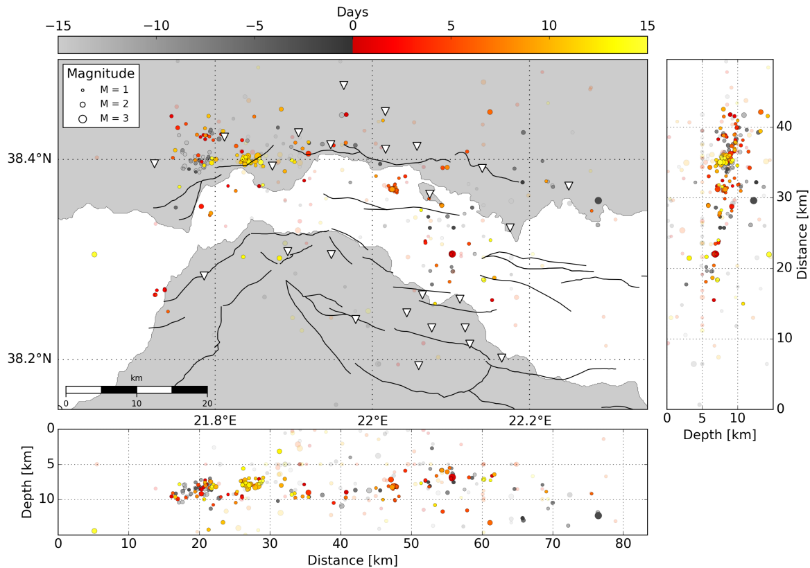
Figure 5.8 – Microseismicity map preceding and following the passing surface waves of the Tohoku earthquake ( M_W 9.0 , 2011). The colorbar is proportional to the time, in gray for events 15 days before the surface wave arrivals and in warm colors 15 days after. Transparent events are non-relocated events. The major faults are mapped in black and the seismic stations are represented by upside-down white triangles.
