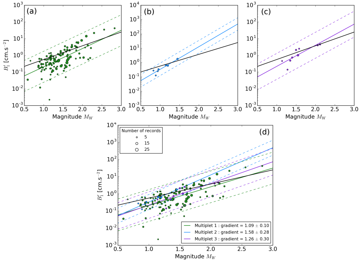
Figure 6.12 – Positive correlation of B'_1 with magnitude on the three multiplets. Slope B'_1 of the linear fit of the first 3 points in the PTW-curves as a function of the magnitude for (a) the large multiplet \mathcal{M}_1 , (b) the multiplet \mathcal{M}_2 linked to pore pressure, (c) the repeater \mathcal{M}_3 . (d) This plot gather the three previous ones. The solid black line shows the best fit linear of the first large dataset ranging magnitude 1 to 5. The colored solid line represent the best linear fit of each dataset. The dashed lines represent the 95% confident intervals.
